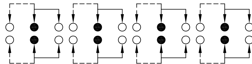
SCHEMATIC (NON-SHORTING)
